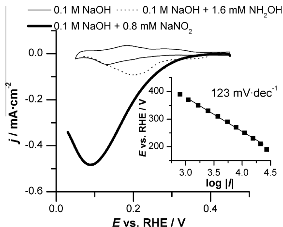
Fig. 6. Comparison of the voltammetric profiles of a stationary Rh electrode in 0.1 M NaOH (blank, thin line), with the addition of 0.8 mM NaNO 2 (bold line) or 1.6 mM NH 2 OH (dotted line). \nu = 20 mV/s. Inset: Tafel slope analysis for a Rh electrode immersed in a 0.1 M NaOH + 0.8 mM NaNO 2 solution. Potential program: steps of 10 mV/min.
