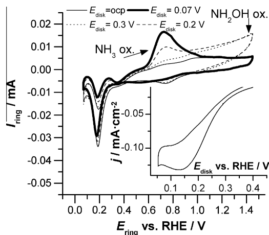
Fig. 5. Profile of the ring current during a shielding experiment ( \omega = 900 rpm, \nu = 10 mV/s) in 0.1 M NaOH + 0.8 mM NaNO 2 . I ring is shown for various E disk values. Inset: current recorded at a Rh disk during potential scan ( \omega = 900 rpm, \nu = 10 mV/s) in 0.1 M NaOH, 50 \mu M NaNO 2 .
