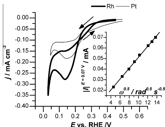
Fig. 2. Reduction profile of 50 \mu\text{M} \text{NaNO}_2 in 0.5 M \text{H}_2\text{SO}_4 at a rotating Rh electrode (bold line) compared to a rotating Pt electrode (thin line), v = 10 \text{ mV/s} , \omega = 900 \text{ rpm} . Inset: Levich plot at E = 0.07 \text{ V} .
