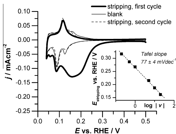
Fig. 1. Voltammetric profile for the first two cycles of adsorbate stripping (bold line, first cycle; dashed line, second cycle) on a polycrystalline Rh electrode in 0.1 M \text{H}_2\text{SO}_4 , v = 20 \text{ mV/s} (blank CV: thin line). Inset: Tafel slope for adsorbate stripping in the same electrolyte.
