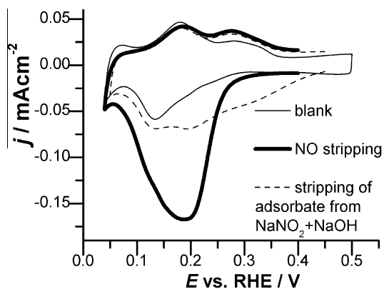
Fig. 7. Voltammetric profile for the stripping of adsorbed NO in 0.1 M NaOH (bold line, first cycle) on a Rh electrode, compared to the stripping (in the same electrolyte) of the adsorbate generated in 0.1 M NaOH + 0.8 mM NaNO 2 (dotted line) and the blank voltammogram (thin line). \nu = 20 mV/s.
