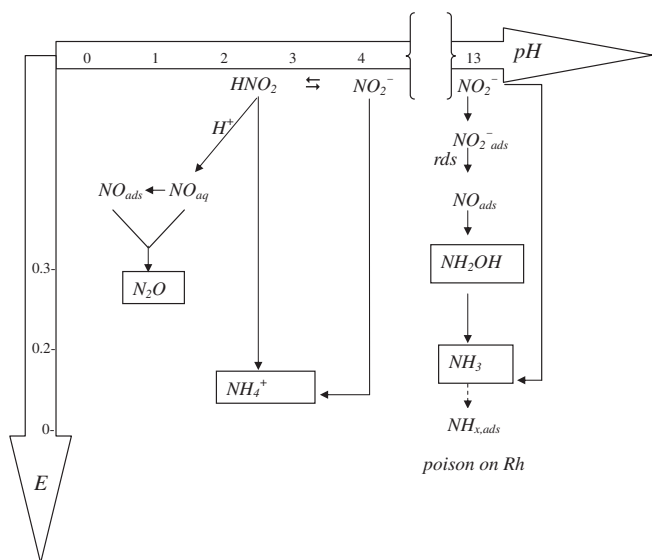
Scheme 1. Mechanistic pathways for \text{NO}_2^-/\text{HNO}_2 reduction at a polycrystalline Rh electrode as a function of pH and E .
