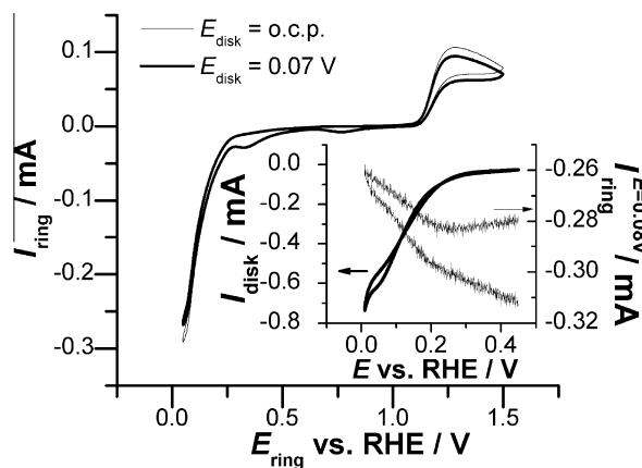
Fig. 3. Profile of the ring current during a shielding experiment ( \omega = 900 rpm, v = 10 mV/s) in 0.5 M \text{H}_2\text{SO}_4 + 0.8 mM \text{NaNO}_2 . Bold line depicts I_{\text{ring}} with E_{\text{disk}} = 0.07 V, and thin line with disk at open circuit potential (o.c.p.). Inset: comparison between the current recorded at a Rh disk ( I_{\text{disk}} , bold line) during potential scan ( \omega = 1200 rpm, v = 10 mV/s) and a Pt ring ( I_{\text{ring}} , E_{\text{ring}} = 0.08 V, thin line) in the same solution as the main figure.
