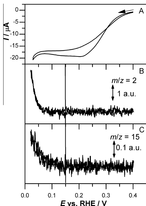
Fig. 8. Cyclic voltammetry during OLEMS measurements (A) and ion current profiles for m/z = 2 (B) and m/z = 15 (C) in 0.1 M NaOH containing 0.8 mM NaNO 2 . The working electrode was a polycrystalline Rh bead electrode, \nu = 1 mV/s. The arrow indicates the beginning of the potential sweep.
